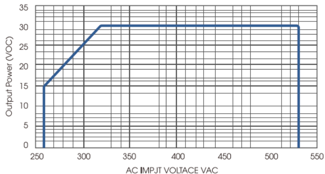
Input Voltage VS Output Power
